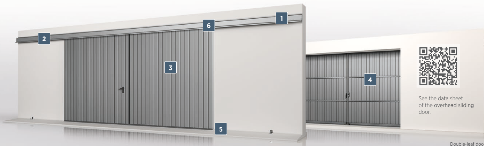
Double-leaf door
